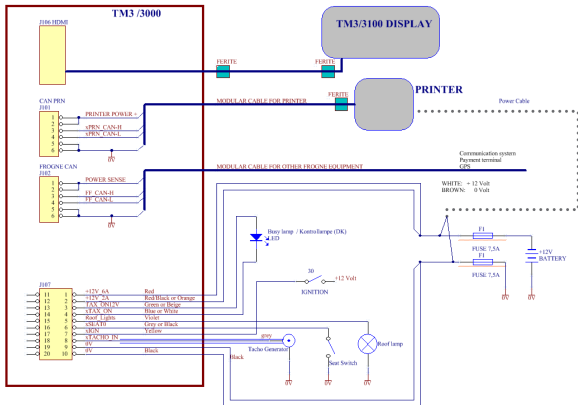
Figure 1: Taximeter connections
