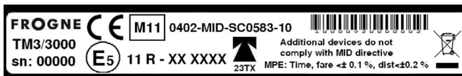
Figure 10: Layout of marking on the CPU
